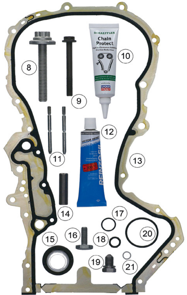
Figure 2: 559 1808 40 / 559 1808 41 - Timing chain KIT attachments
