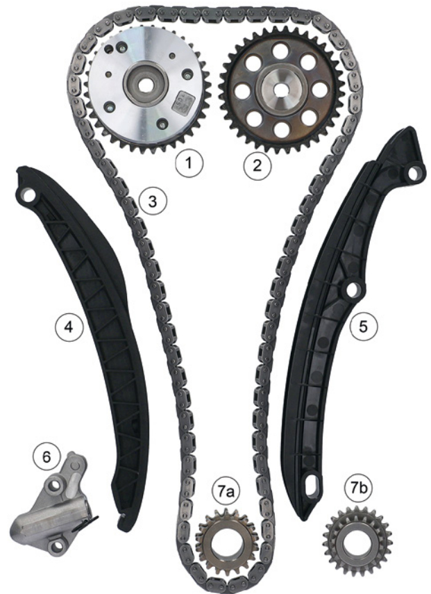
Figure 1: 559 1808 40 / 559 1808 41 – Timing chain KIT components
